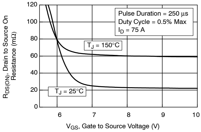
Figure 11. R_{DS(on)} vs. Gate Voltage
