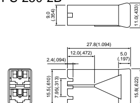
PS-250-2B
