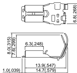
SFPS-41T-187...for 0.5mm(.020")
