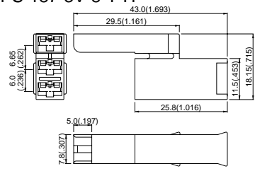
PS-187-3V-8-T-H
