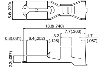
SPS-82T-187...for 0.5mm(.020")
